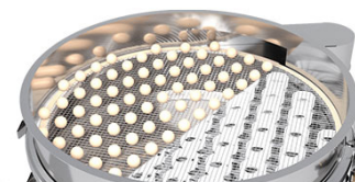
Self-cleaning ring/food-grade rubber balls
